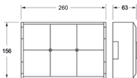
Compact in size: W 260 x D 156 x H 63 mm.
